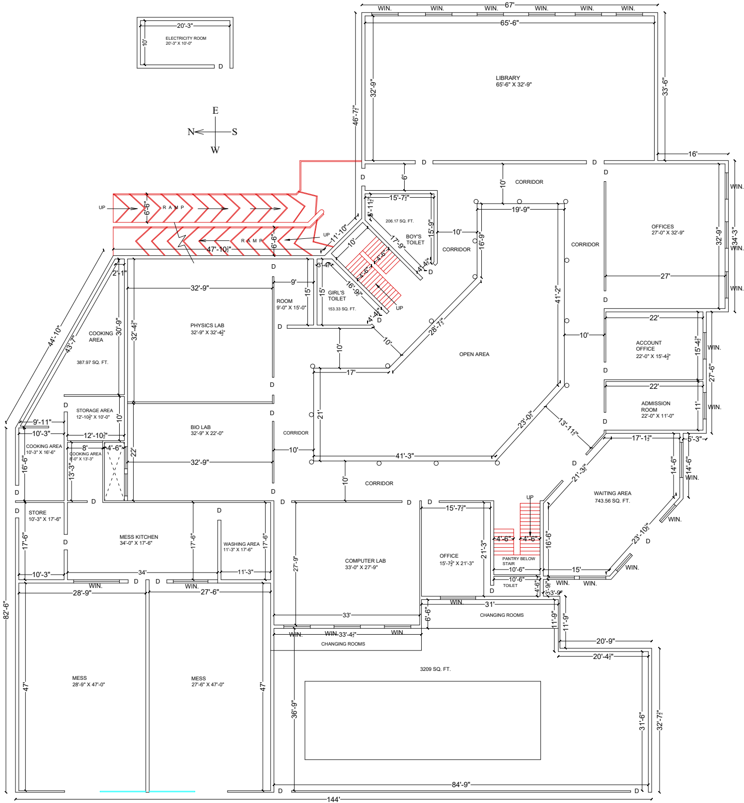
GROUND FLOOR PLAN ( 19690 SQ. FT.)
