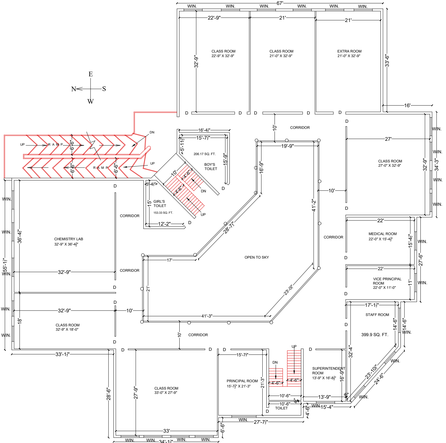
FIRST FLOOR PLAN (11390.375SQ. FT.)
